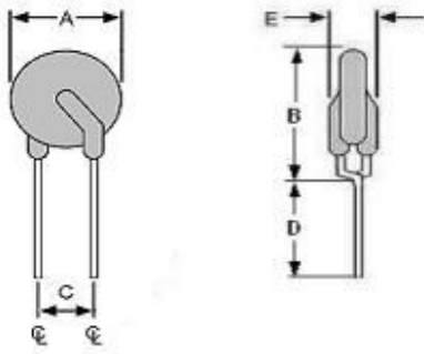
Fig.1 Lead Size :22AWG, Φ 0.65 mm Diameter
