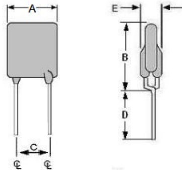
Fig.2 Lead Size : 22AWG, Φ 0.65 mm Diameter
